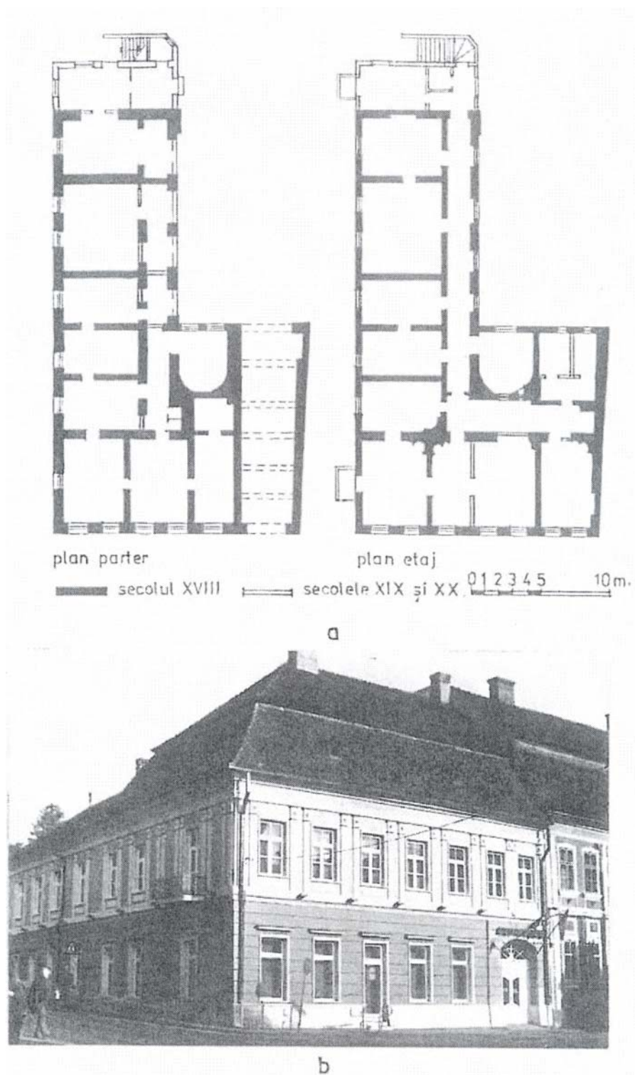
Fig. 107. Casa Haller. a – Plan nivele; b – Aspect general.
